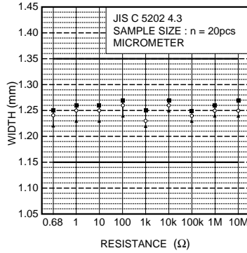
Fig.3 Dimensions (width)
