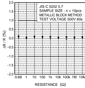
Fig.9 Withstand voltage
