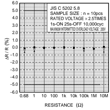
Fig.10 Intermittent overload
