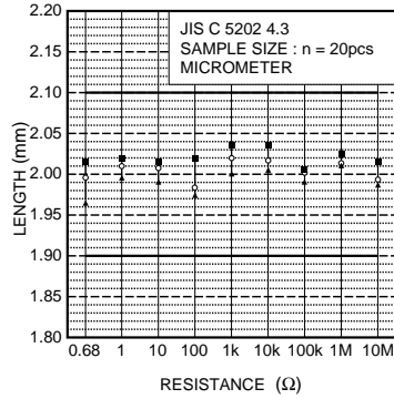
Fig.2 Dimensions (length)
