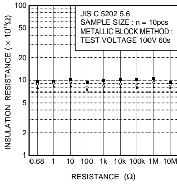
Fig.8 Insulation resistance
