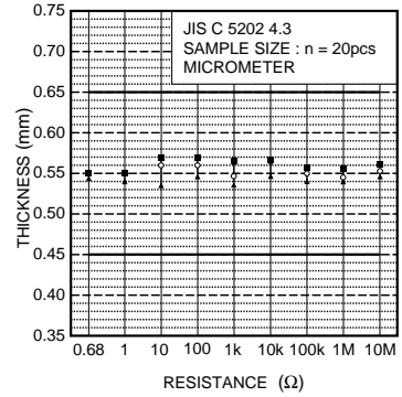
Fig.4 Dimensions (thickness)
